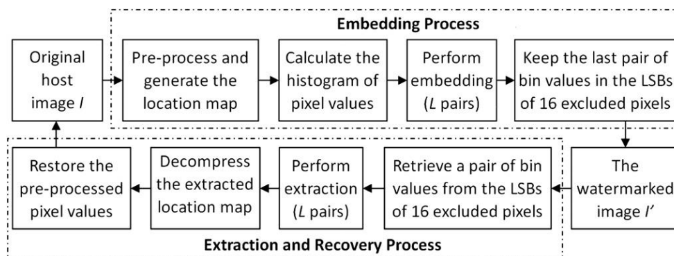
Figure 1: Procedure of the proposed RDH algorithm [1]
